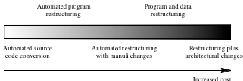
Figure 28.3 Re-engineering approaches
